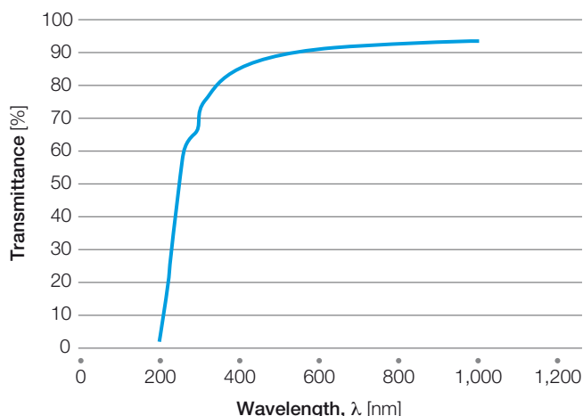
Figure 11: Absorption spectra of Halar® 500 in UV and visible ranges
