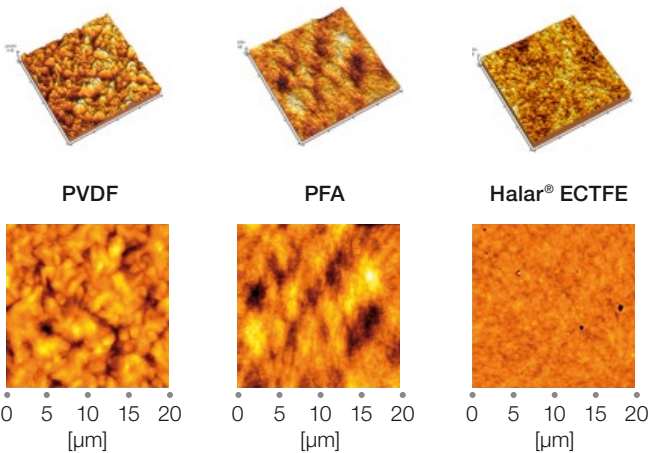
Figure 9: Atomic Force Microscopy topographies of the inside surface of fluoropolymers extruded pipes
