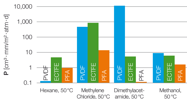
Figure 35: Liquid permeabilities of a few common chemicals in Halar® ECTFE, compared with other fluoropolymers
