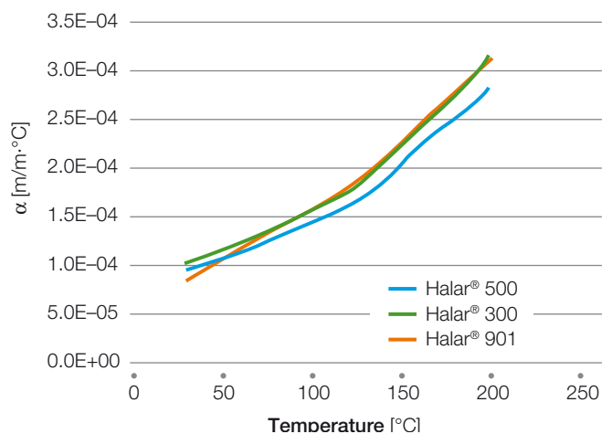
Figure 3: Thermal expansion curves for Halar® ECTFE measured by thermomechanical analysis (TMA)
