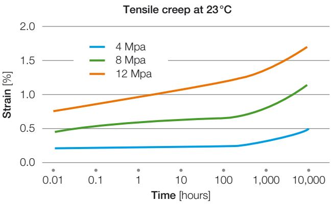
Figures 18, 19, 20 and 21: Tensile creep of Halar® ECTFE at various temperatures and under different stresses
