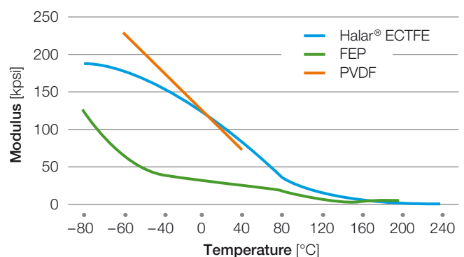
Figure 17: Compressive modulus for Halar® ECTFE and other fluoropolymers
