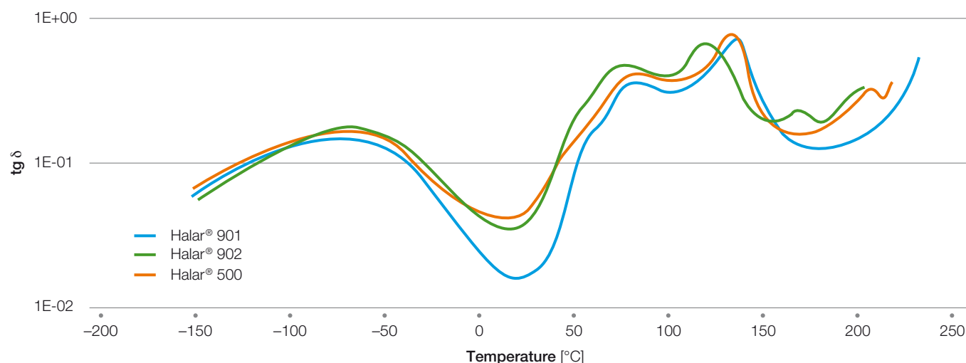
Figure 25: Damping (or \tan \delta ) of Halar® ECTFE copolymers vs. temperature (DMTA)
