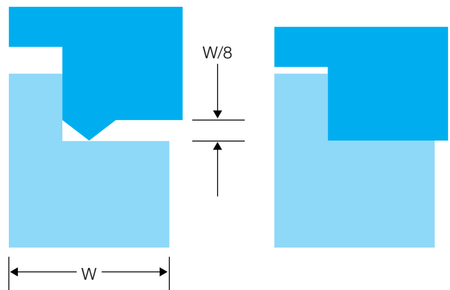
Figure 2: Step joint
