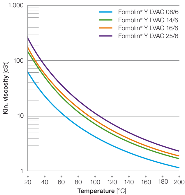
Fomblin® Y LVAC – kinematic viscosity vs. temperature
