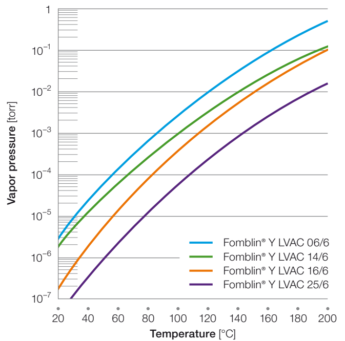
Fomblin® Y LVAC – vapor pressure vs. temperature
