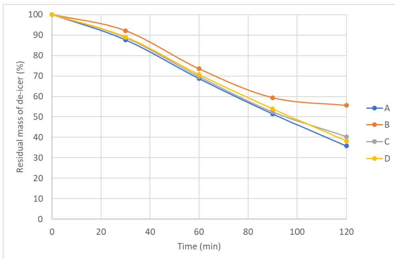
Figure 3 – Residual mass of de-icer solutions on road replica surface during a simulation of an approaching cold front. Temperature was kept at 10 °C and the relative humidity fell from 80 % to 20% between t=30 min. and t=120 min.
