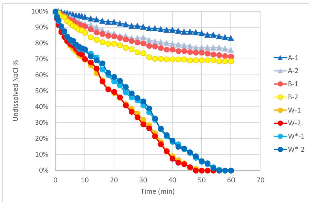
Figure 1 – Dissolution of NaCl in solution A, B and water (W) at 22 °C. Dissolution of NaCl in water at 5 °C (W*).
