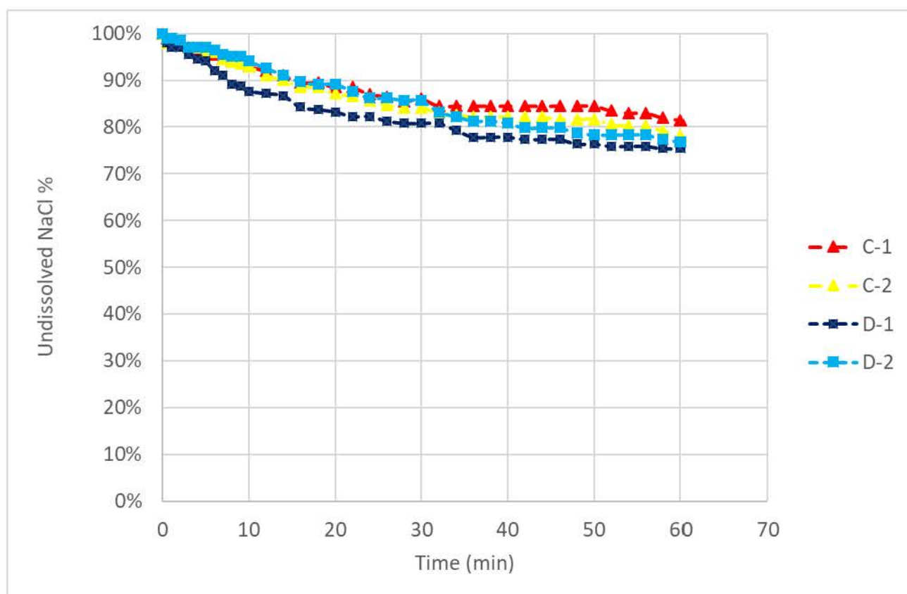
Figure 2 – Dissolution of NaCl in solution C and D at 22 °C.
